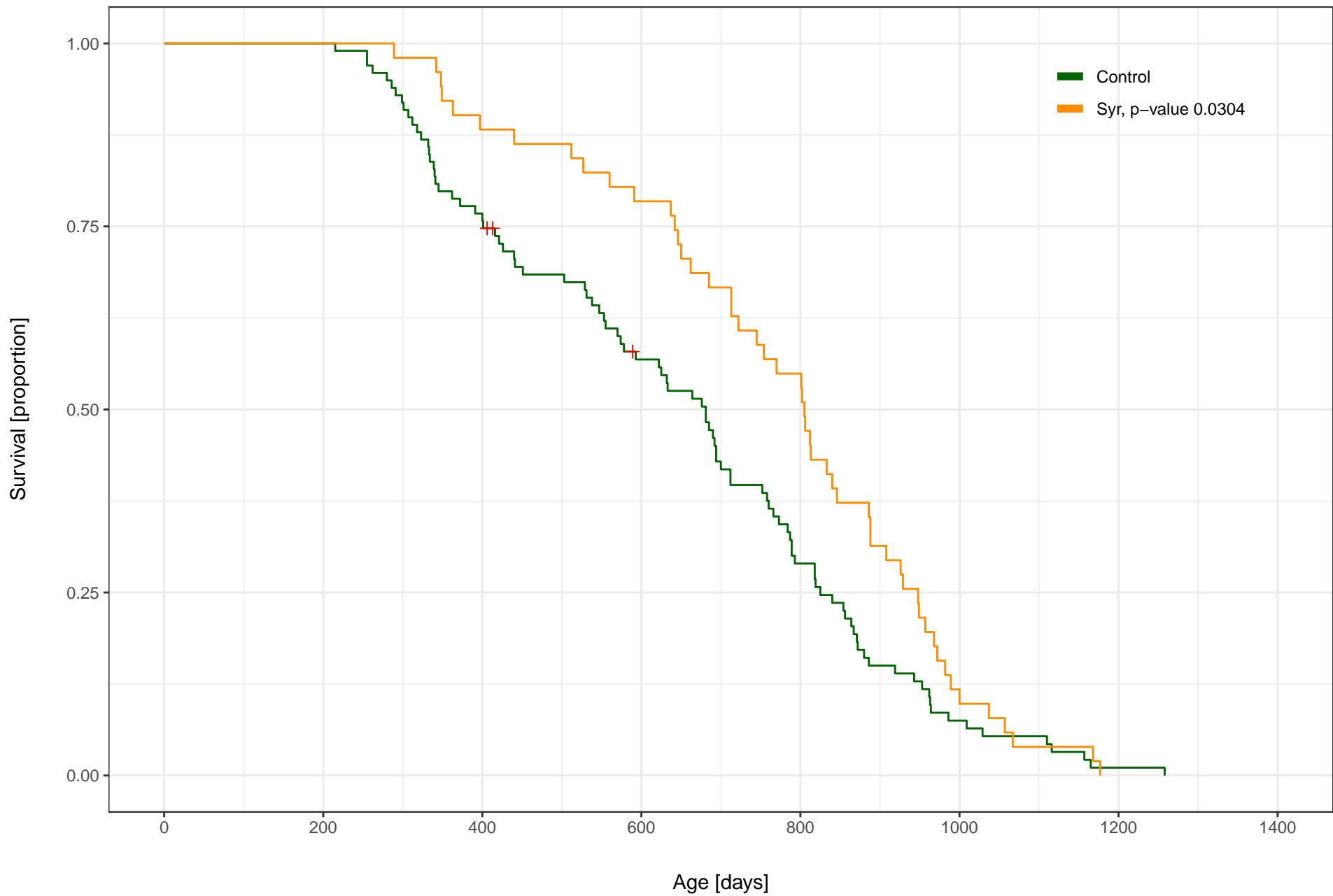
syringaresinol (300 ppm) vs. Control, Male, C2017 UT
