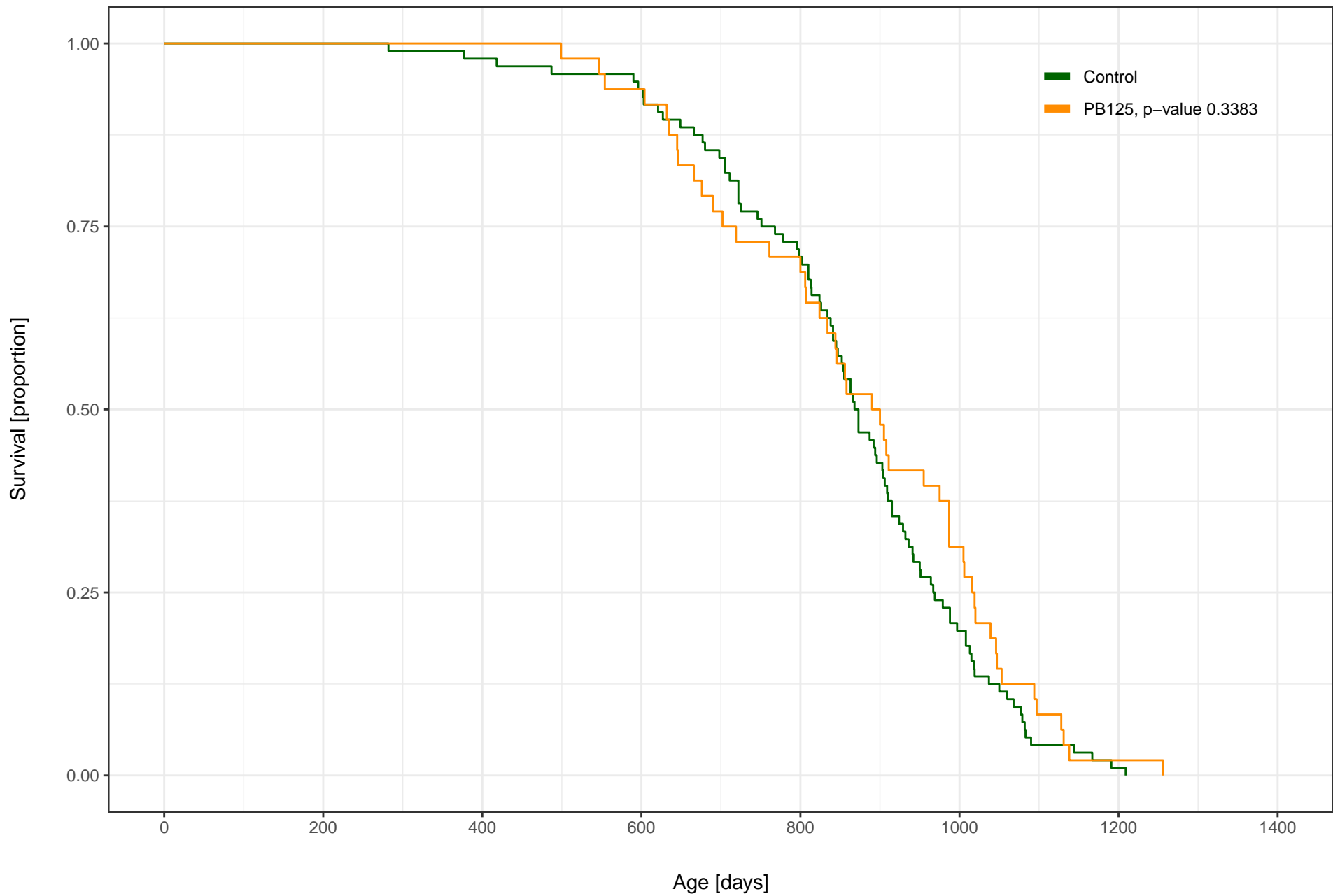
PB125 (see publication ppm) vs. Control, Female, C2017 TJL
