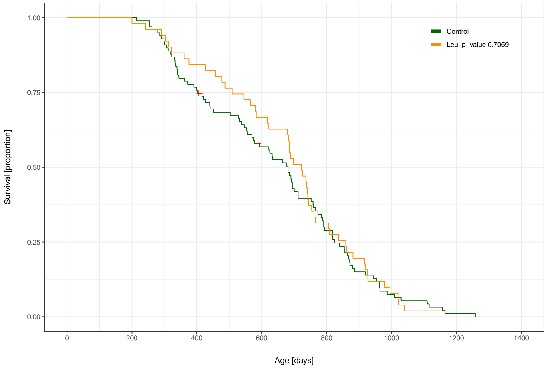
L-leucine (40000 ppm) vs. Control, Male, C2017 UT
