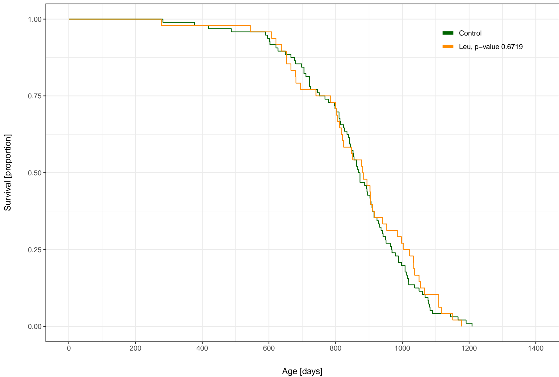
L-leucine (40000 ppm) vs. Control, Female, C2017 TJL
