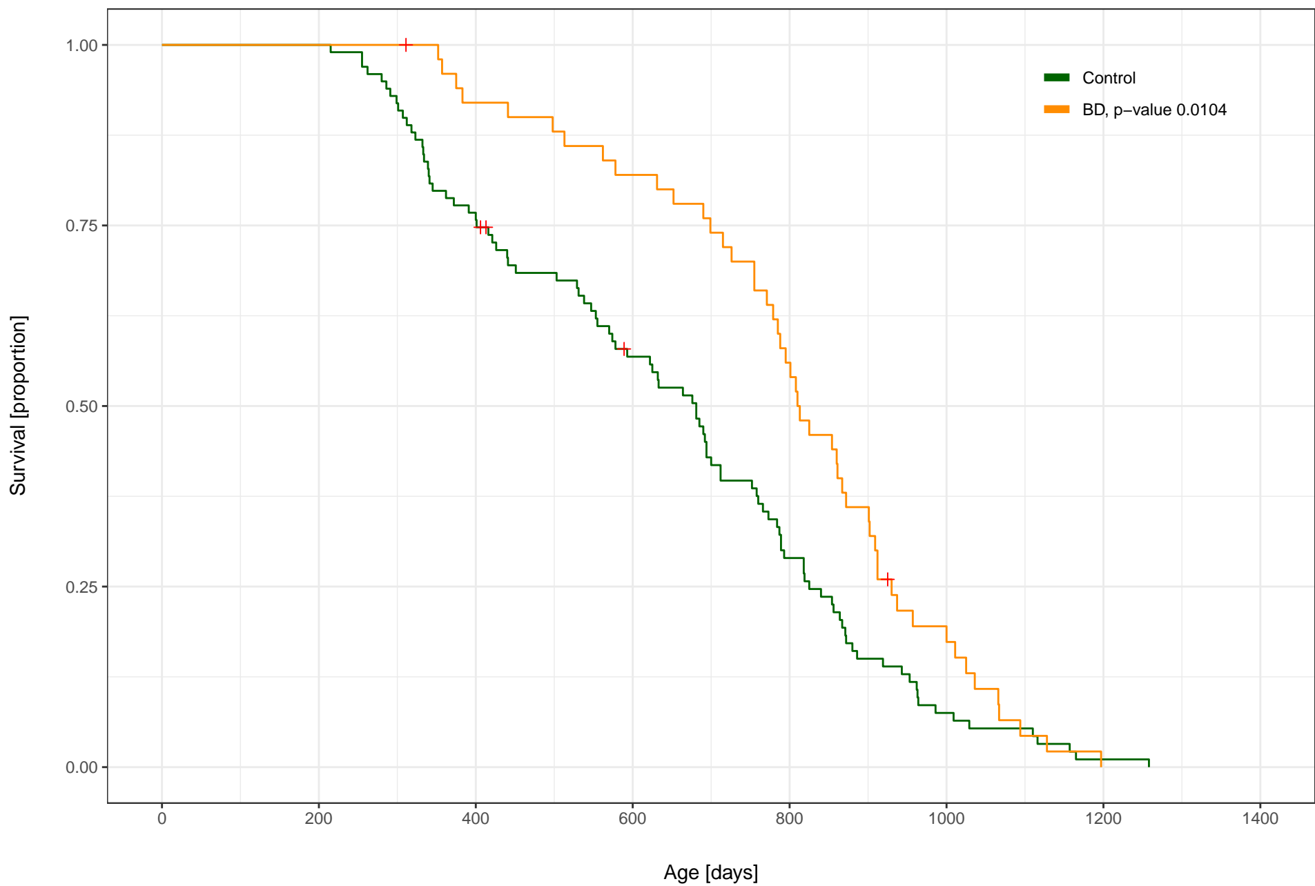
(R/S)-1,3-butanediol (100000 ppm) vs. Control, Male, C2017 UT
