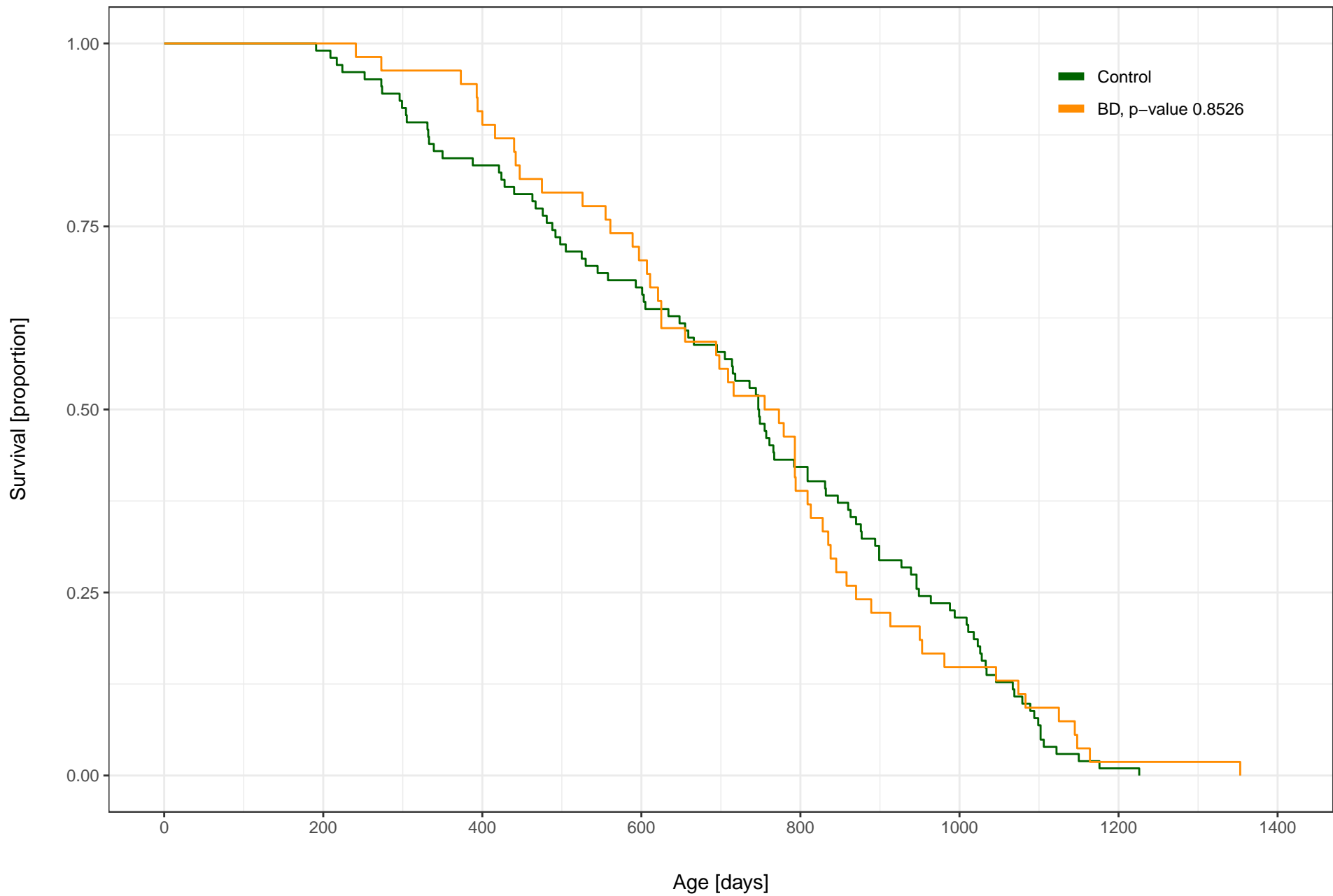
(R/S)-1,3-butanediol (100000 ppm) vs. Control, Male, C2017 TJL
