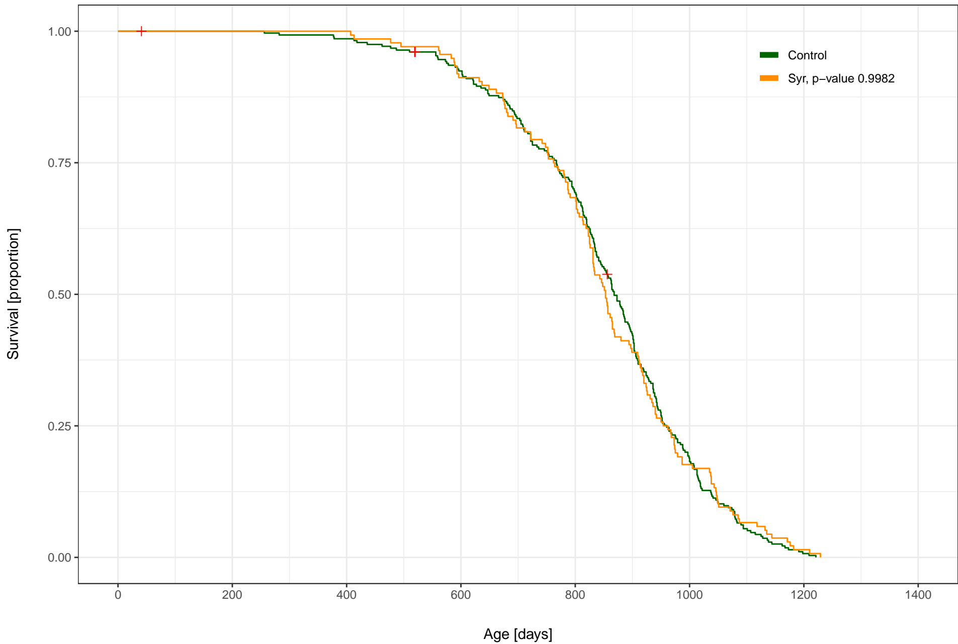
syringaresinol (300 ppm) vs. Control, Female, C2017 All Sites
