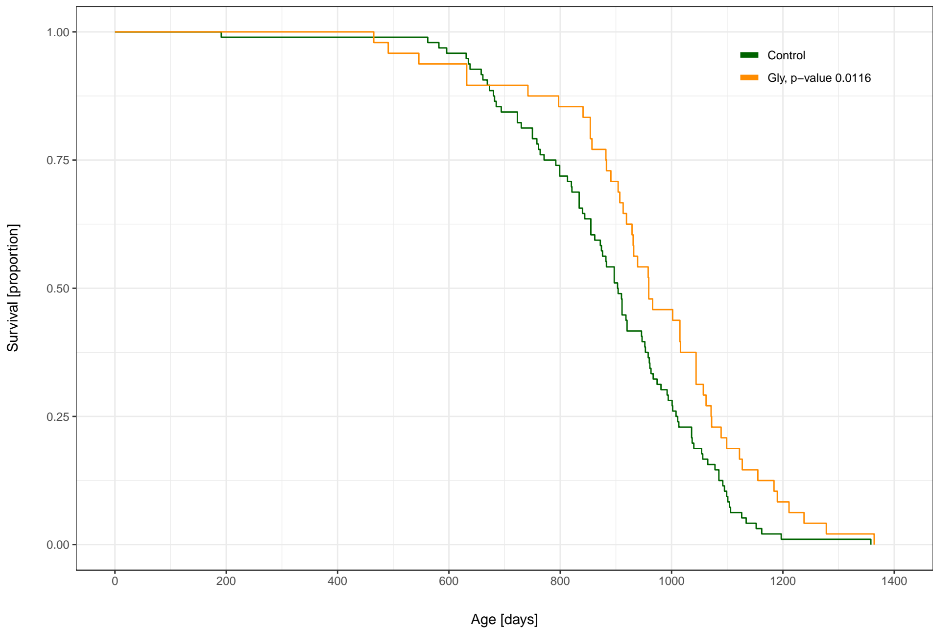
Gly (80,000 ppm) vs. Control, Female, C2014 TJL
