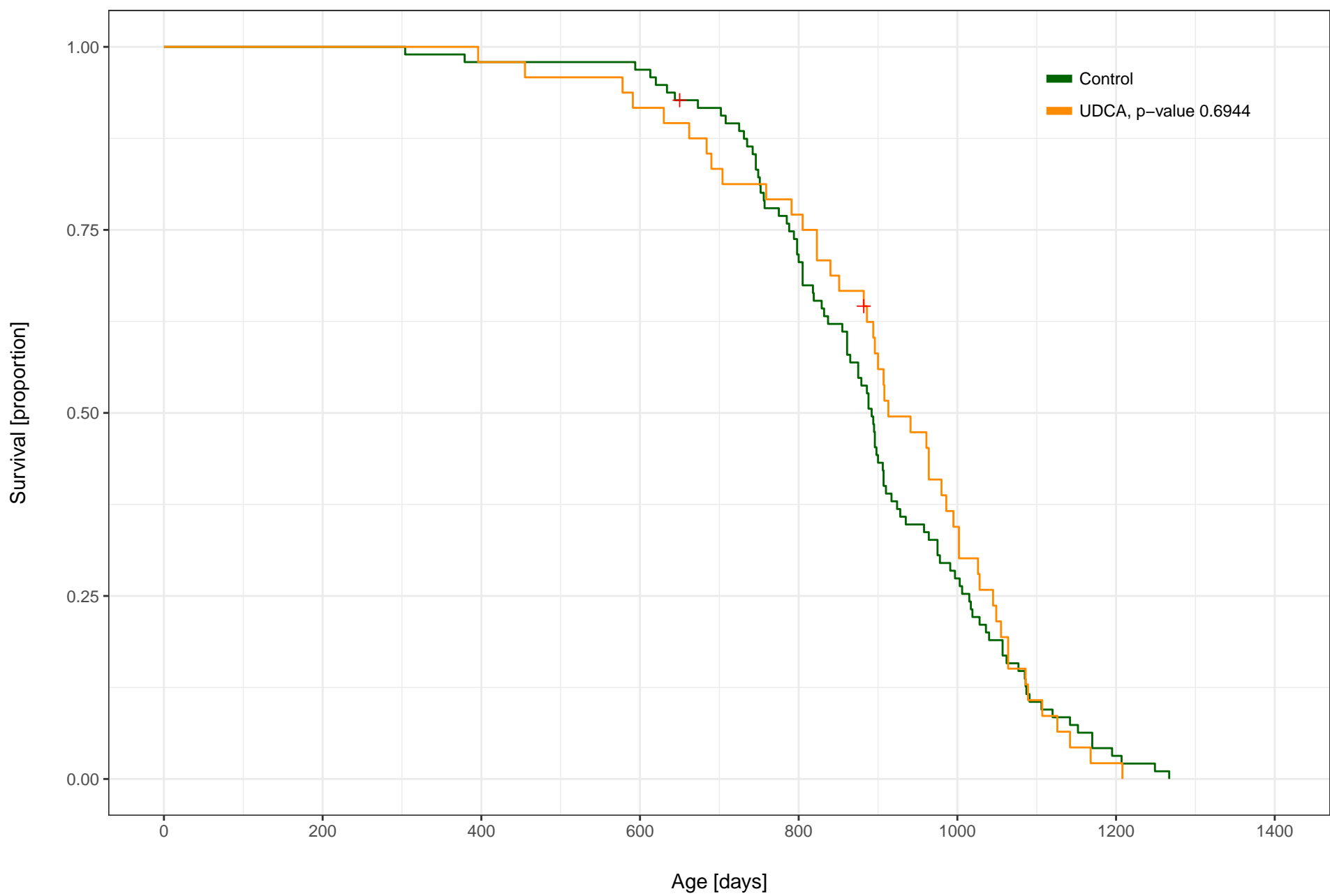
UDCA (5000 ppm) vs. Control, Female, C2011 TJL
