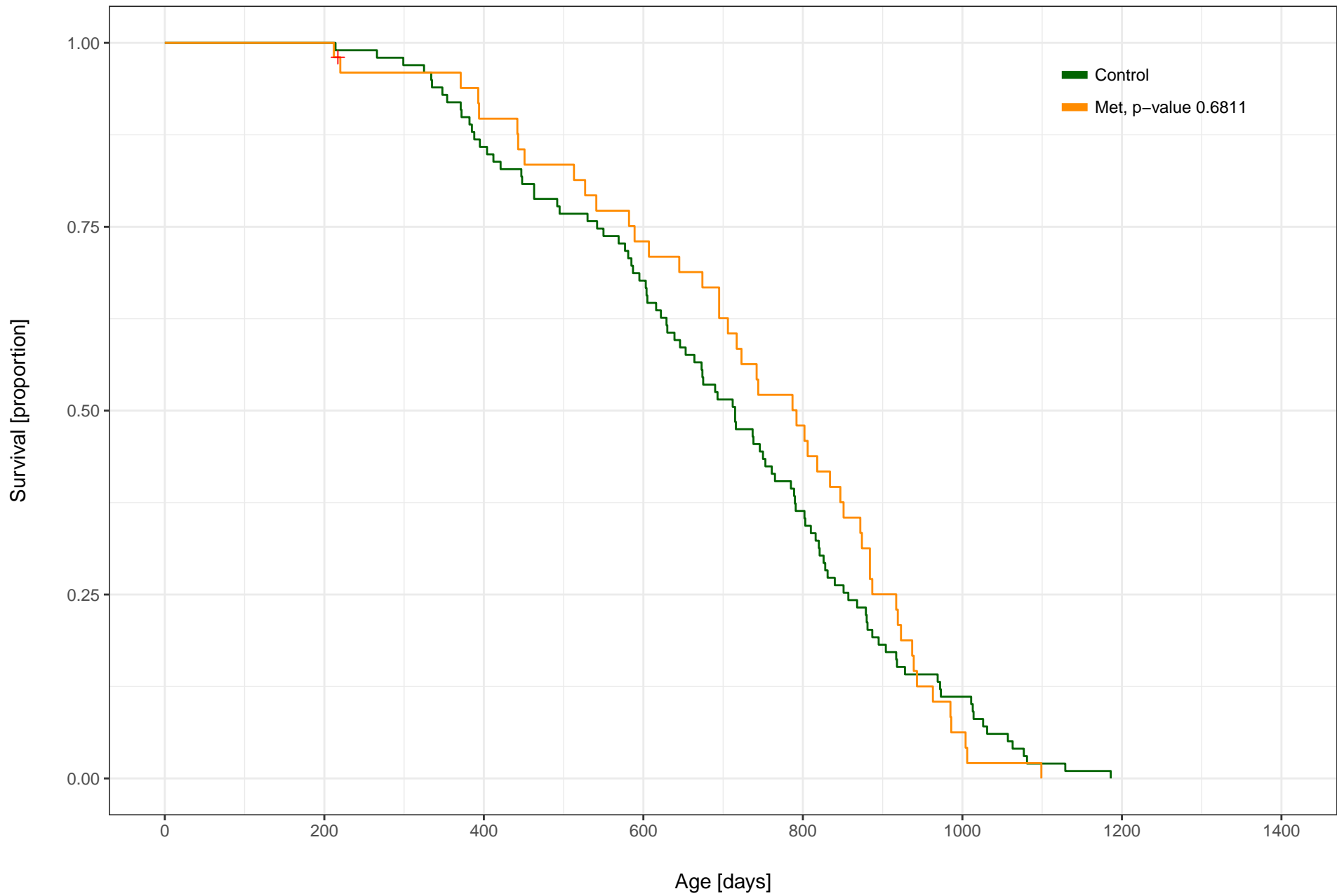
Met (1000 ppm) vs. Control, Male, C2011 UT
