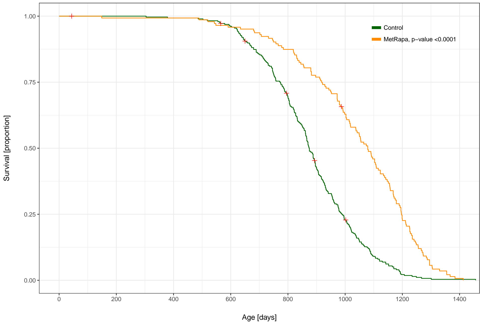
MetRapa (1000, 14 ppm) vs. Control, Female, C2011 All Sites
