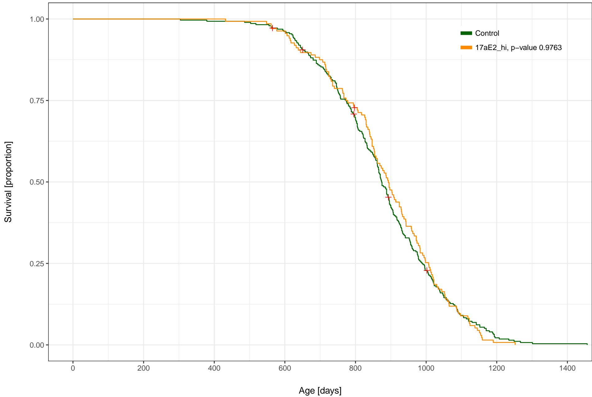
17aE2 (14 ppm) vs. Control, Female, C2011 All Sites
