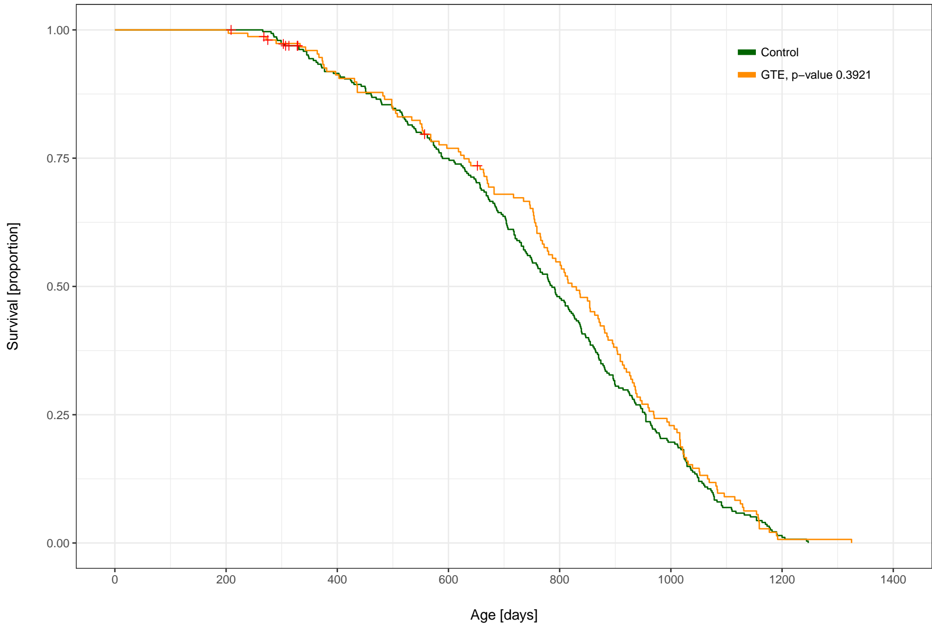
GTE (2000 ppm) vs. Control, Male, C2007 All Sites
