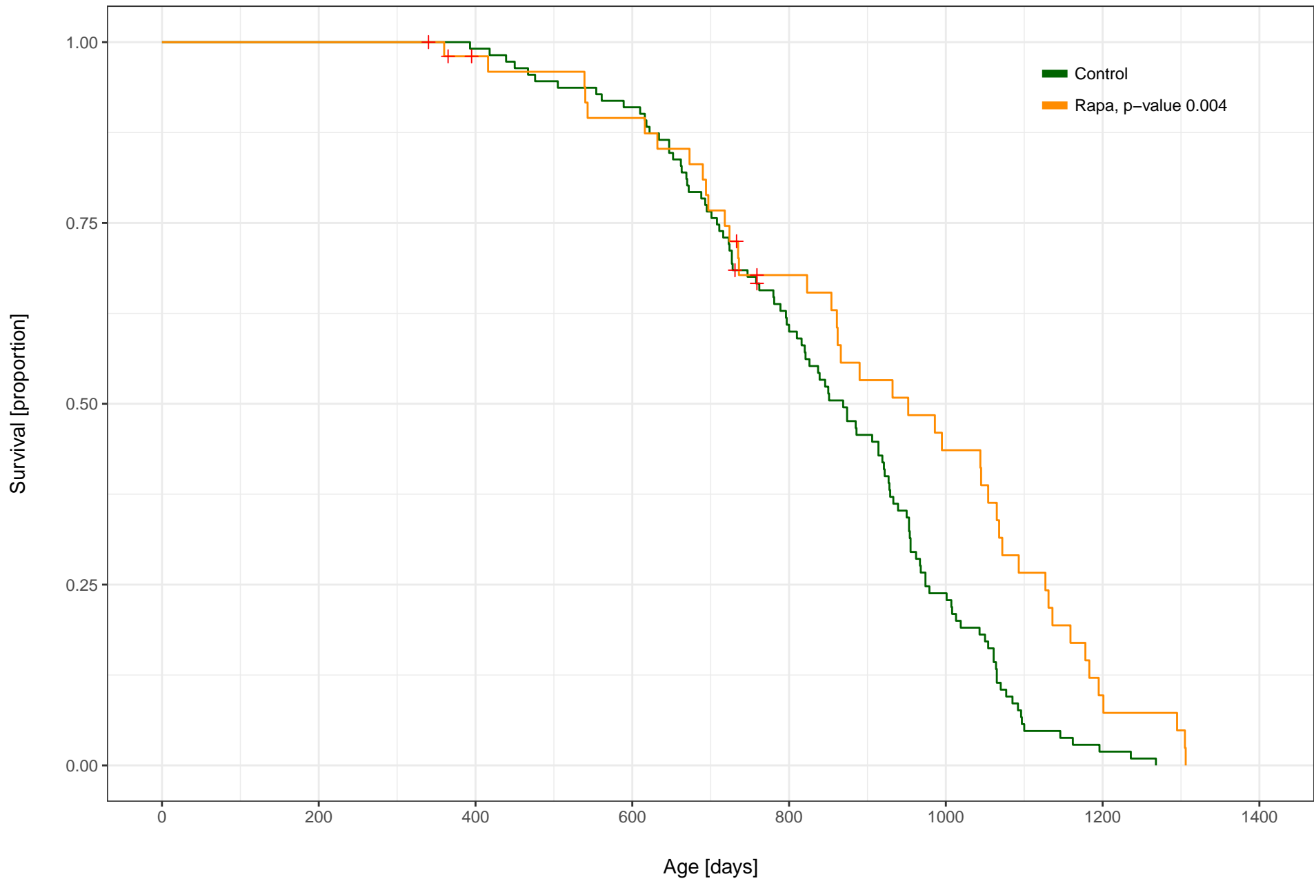
Rapa (14 ppm) vs. Control, Male, C2006 UM
