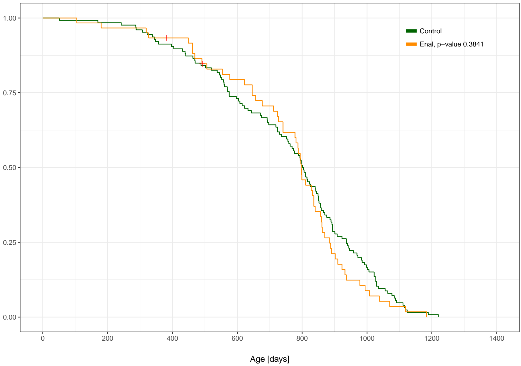
Enal (120 ppm) vs. Control, Male, C2005 TJL
