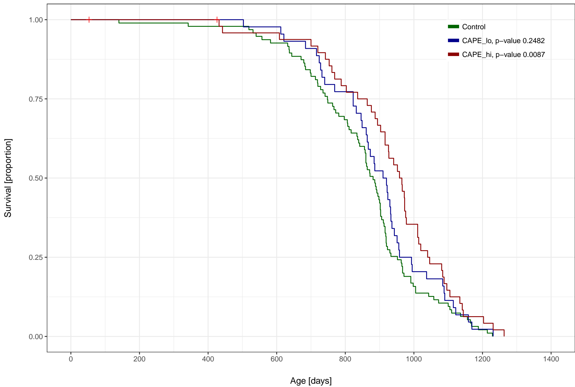
CAPE vs. Control, Female, C2005 TJL
