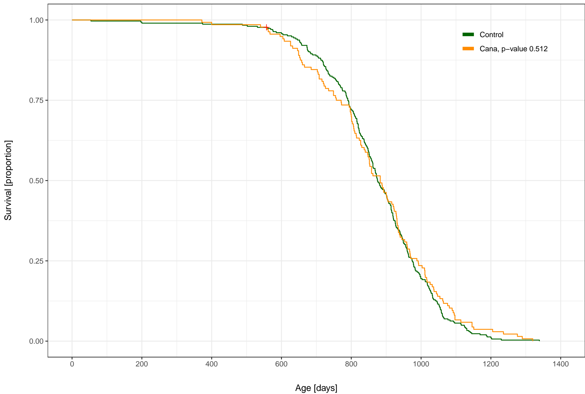
Canagliflozin (180 ppm) vs. Control, Female, C2016 All Sites
