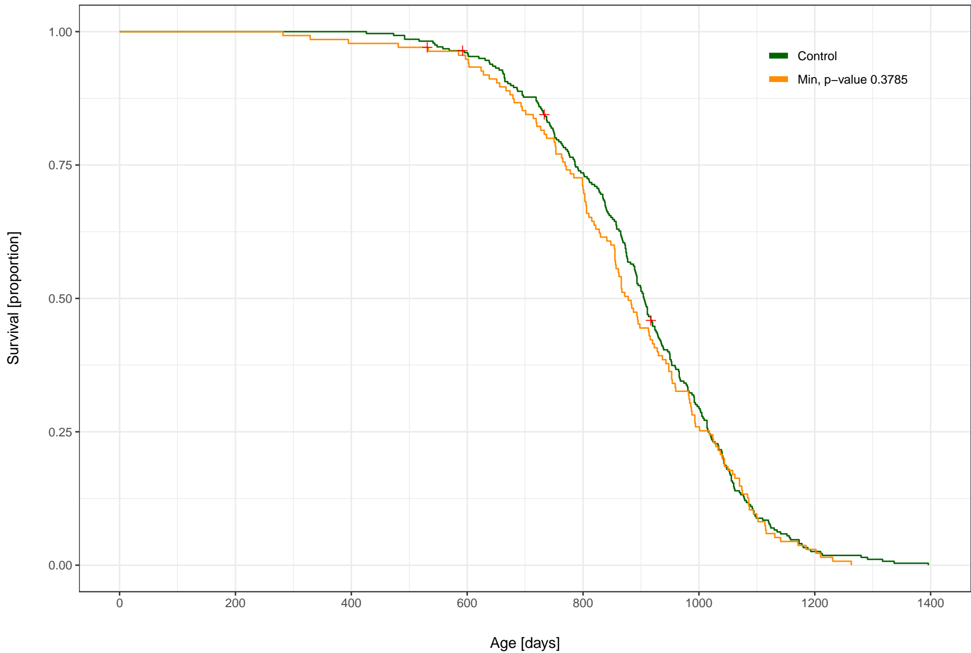
minocycline (300 ppm) vs. Control, Female, C2015 All Sites
