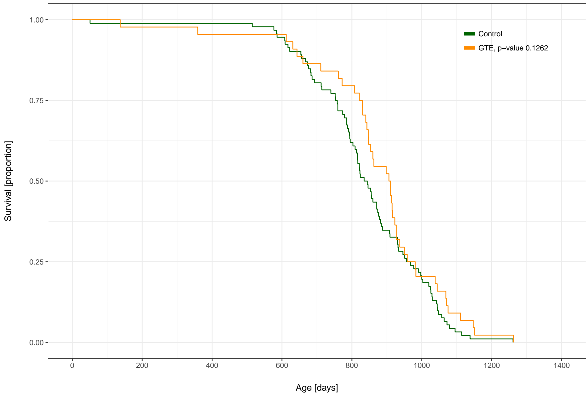
GTE (2000 ppm) vs. Control, Female, C2007 UT
