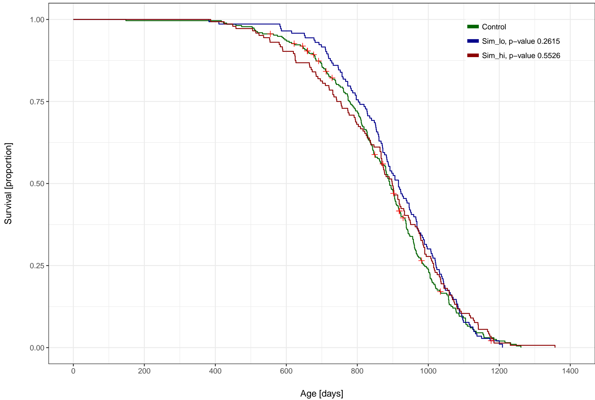
Sim vs. Control, Female, C2006 All Sites
