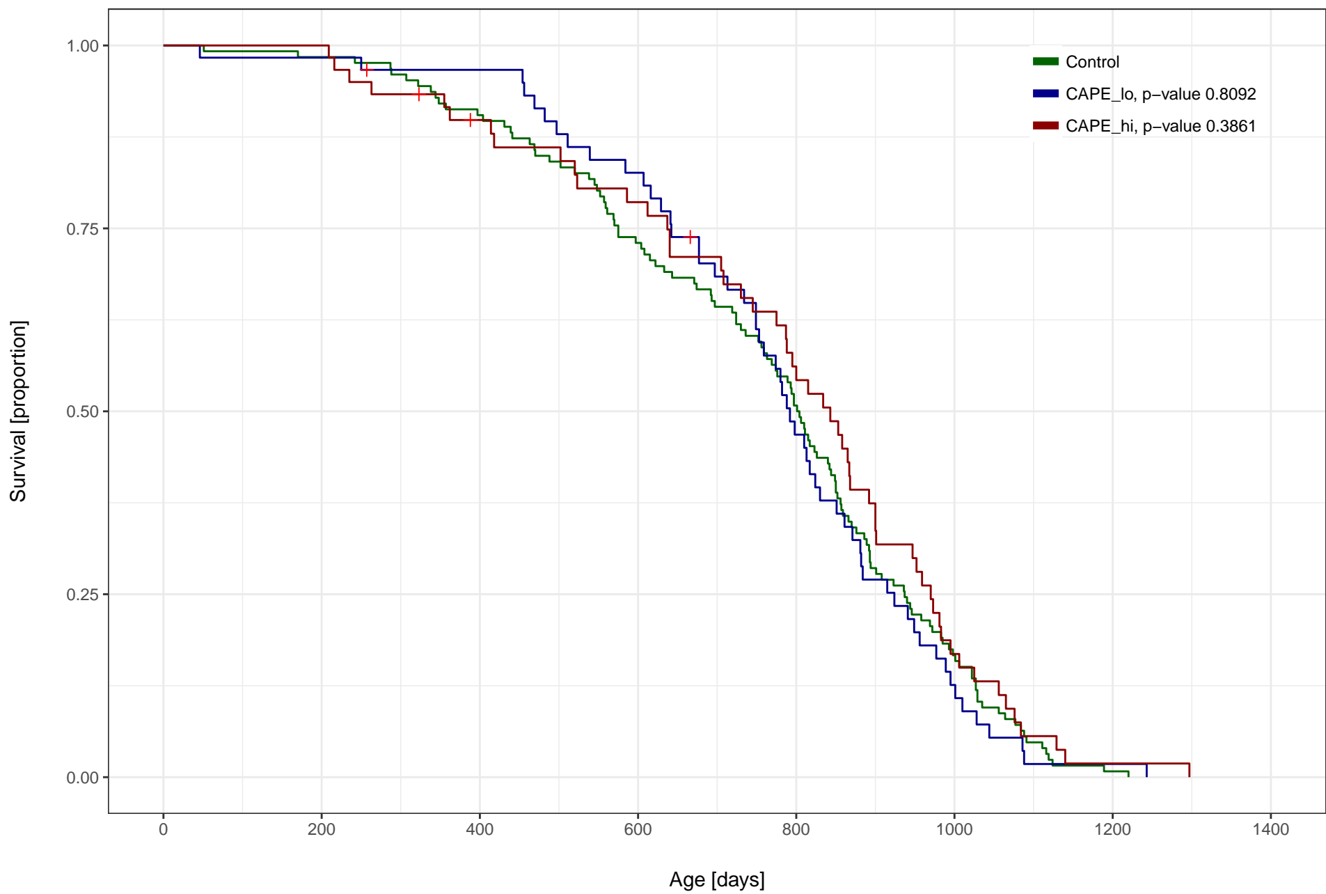
CAPE vs. Control, Male, C2005 TJL
